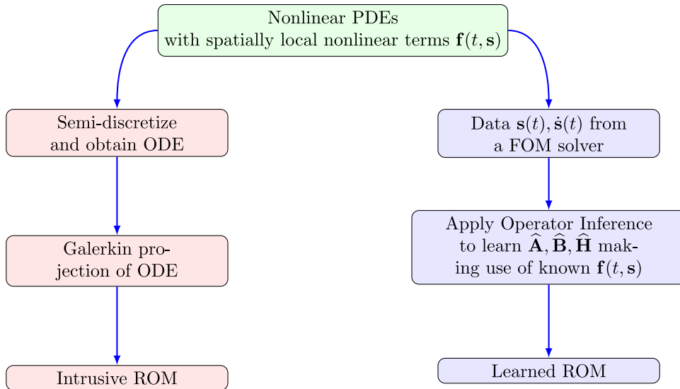
Fig. 1. A comparison of a fully intrusive ROM approach with the proposed learning approach.
