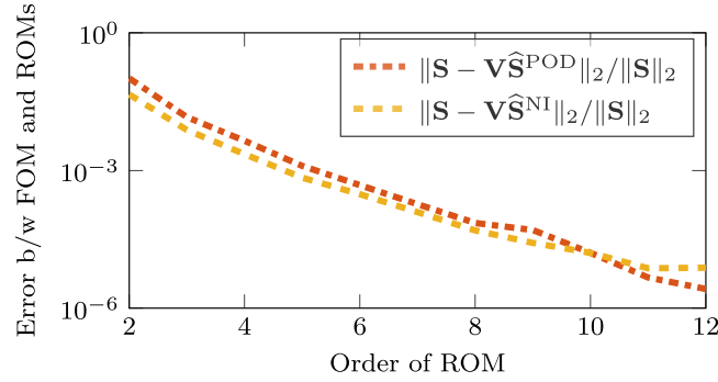
Fig. 4. Chafee–Infante example: Convergence of relative state errors with increasing order of the POD intrusive ROMs and the learned ROMs.
