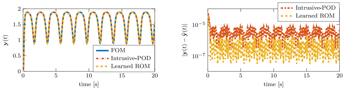
Fig. 3. Chafee–Infante example: Output (left) and output errors (right) of the POD intrusive and the learned ROMs of order r = 12 .
