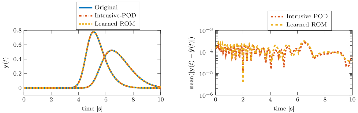
Fig. 10. Batch chromatography example: A comparison of the POD intrusive model with the learned model of order r = 4 \times 22 .
