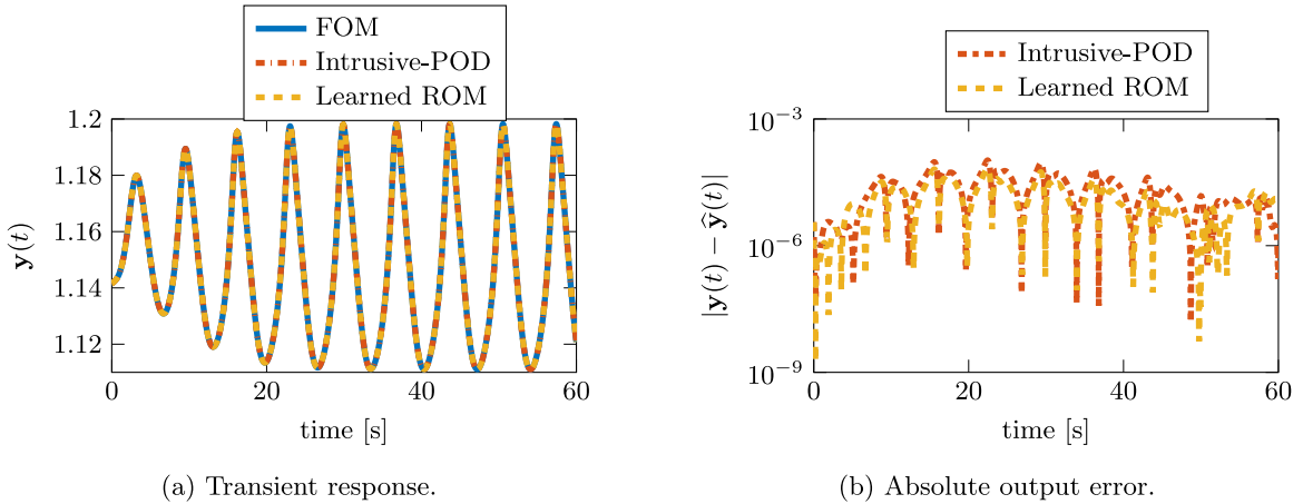
Fig. 6. Tubular reactor example: A comparison of the transient behavior of the projection-based POD ROM and the learned ROM.
