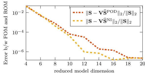
Fig. 7. Tubular reactor example: Relative state errors produced by both ROMs, i.e., \|S - \widehat{V}S^{\text{POD}}\|_2/\|S\|_2 and \|S - \widehat{V}S^{\text{NI}}\|_2/\|S\|_2 .
