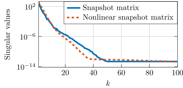
Fig. 5. Tubular reactor example: Decay of the singular values of the snapshot matrix and the nonlinear snapshot matrix.
