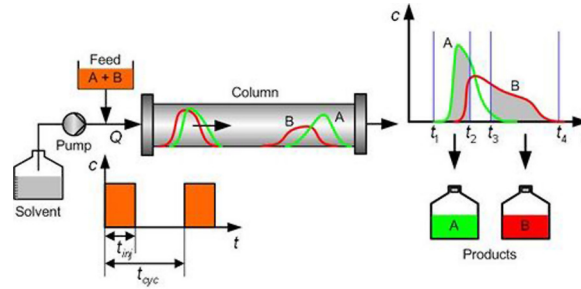
Fig. 8. The figure shows a chromatography process, separating a mixture, c.f. [48].
