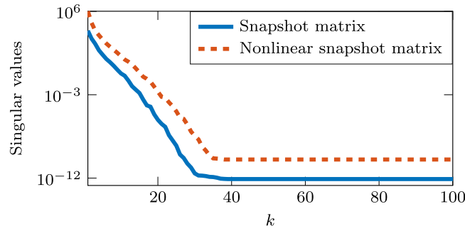
Fig. 2. Chafee–Infante example: Decay of singular values of the snapshot matrix and the nonlinear snapshot matrix.
