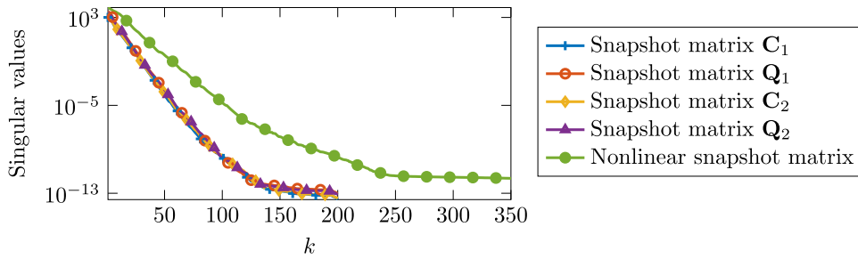
Fig. 9. Batch chromatography example: Decay of singular values of the collected snapshots for all four components separately and the nonlinear snapshot matrix.
